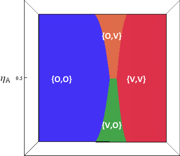
\alpha = 0.9, \beta = 0.8
