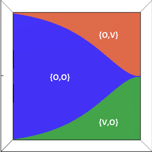
\alpha = 0.7, \beta = 0.4
